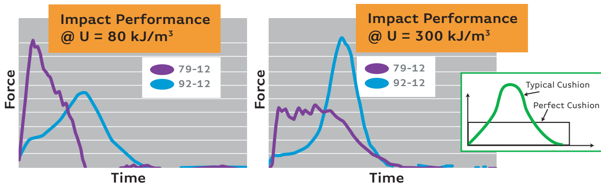
Figure 3: Force vs Time graphs of 92-12 and 79-12 at two different impact energy densities. In each case, the material which can more evenly spread out the impact over time results in a lower peak force. Finally, notice the flatness of the 79-12 curve at U=300 \text{ kJ/m}^3 . It infers that 79-12 behaves similarly to a perfect cushion in this drop condition.
