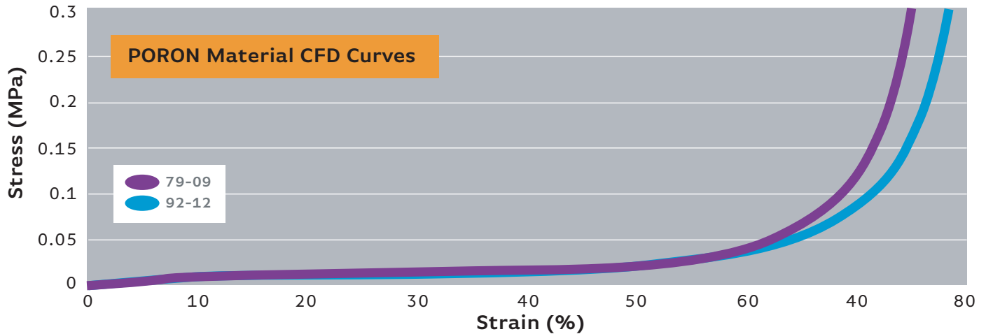
Figure 4: CFD curves of 79-09 and 92-12 materials
