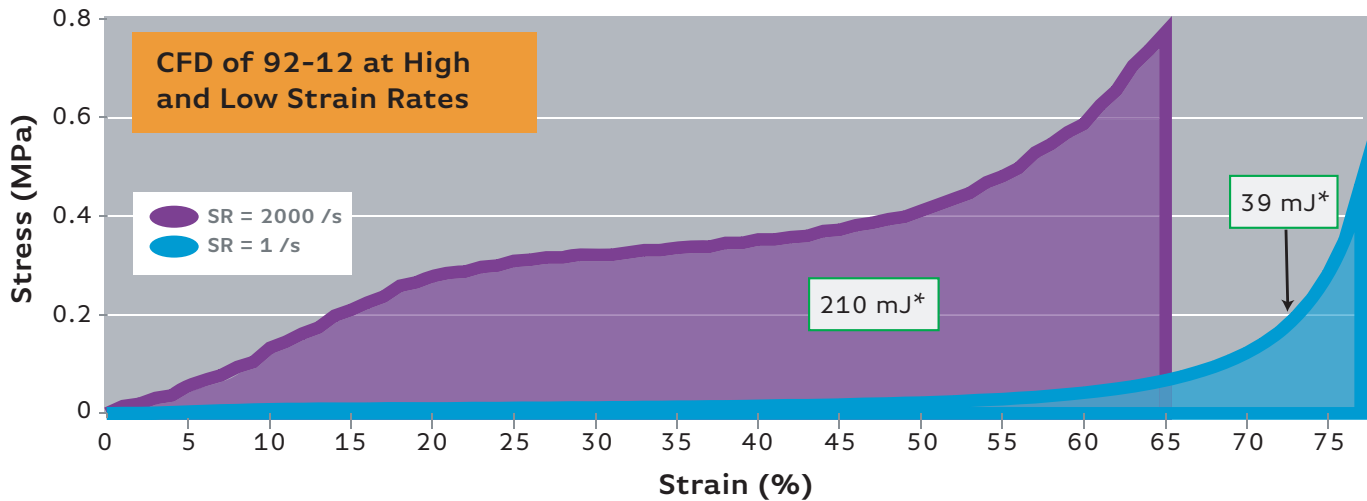
Figure 6: CFD Curves of 92-12 at two different Strain rates, at 1 /s and at 2000 /s. Notice that the area under the high strain rate curve is more than five times that of the area underneath the low strain rate curve.
