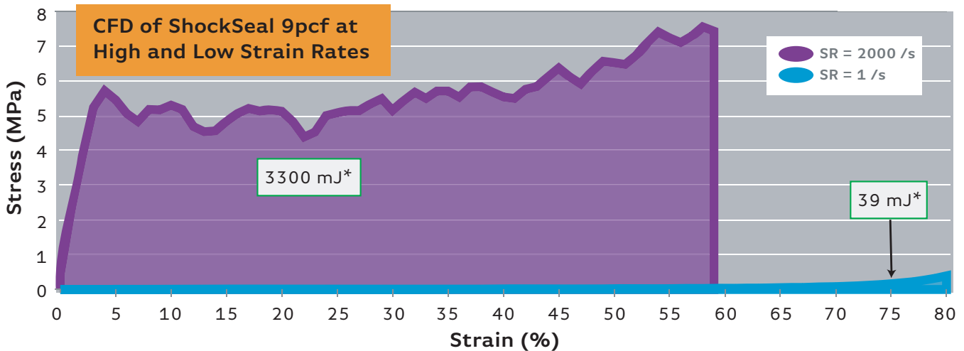
Figure 7: CFD Curves of 79-09 at two different Strain rates, at 1 /s and at 2000 /s. According to these CFD curves the elastic potential of 79-09 materials at 2000 /s is 100 times its elastic potential at 1 /s.
