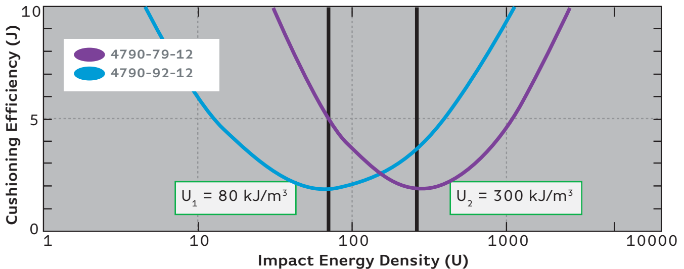
Figure 2: The J-U curves of two materials, 79-12 and 92-12. 79-12 materials cushion higher energy impacts better than 92-12 materials. Additional J-U curves of PORON materials can be found at http://www.rogerscorp.com/impactprediction .
