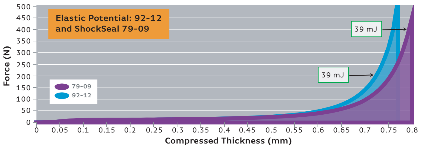
Figure 5: Compression Force vs Compressed Thickness. In this example, a 1 mm in thickness and 1140 mm 2 in area sample was used to calculate these values. These curves demonstrate the elastic potential energy of 92-12 and ShockSeal 79-09 foams.
