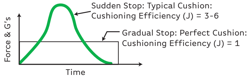
Figure 1: Force vs. Time curves depicting an object striking a typical cushion and a perfect cushion
